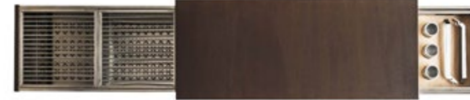
SNAIL #CorTen
